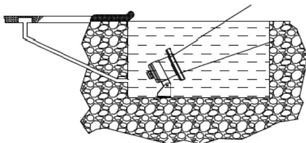
Installation Diagram for F20A Series
